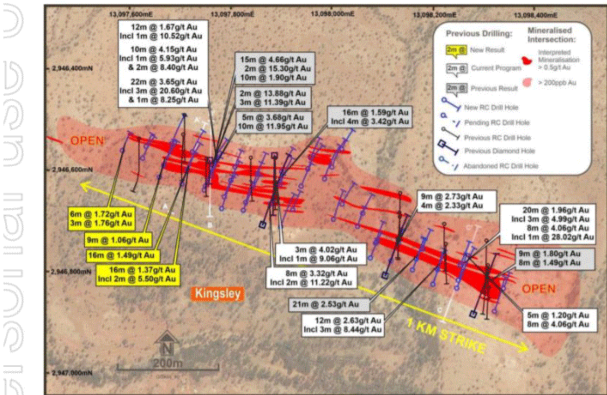
Figure 1: Kingsley Prospect showing strike extent of interpreted mineralised trends and drilling with significant intercepts
