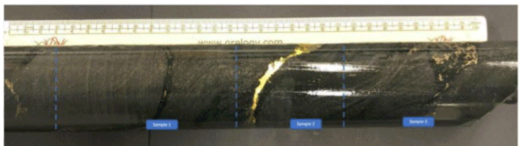
Figure 2: The selected core indicating the three sub-samples
