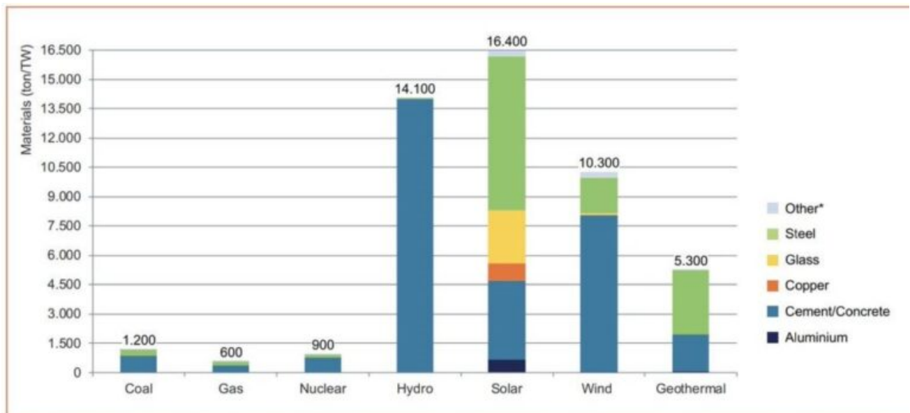
Figure 4: Base-Material Input per 1 TW Generation
