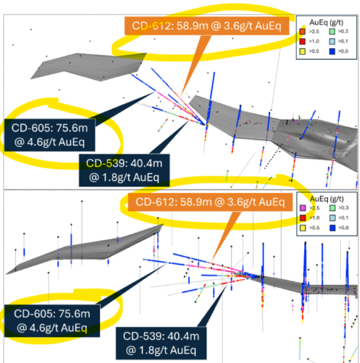
Figure 2: Longitudinal view looking north (top) and plan view (bottom),
